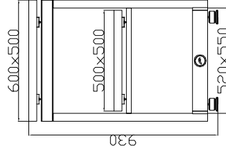
"C" TOP BEAMS RACK
