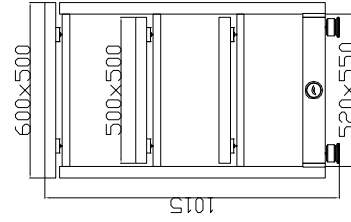
"S" TOP BEAMS RACK
