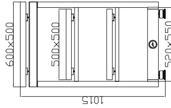
"C" TOP BEAMS RACK
