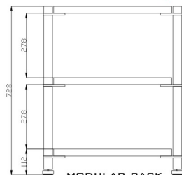
MODULAR RACK RS3 /CODE - MR-RS3/
