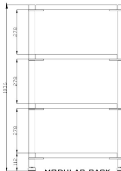
MODULAR RACK RS4 /CODE - MR-RS4/
