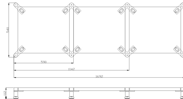
MODULAR RACK RS3 /CODE - MR-RS3/
