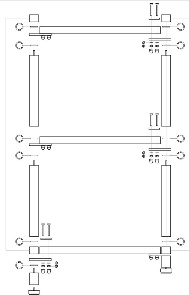
MODULAR RACK RS3 /CODE - MR-RS3/
