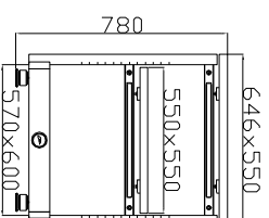
3 LEVELS, 3 COMPONENTS RACK CODE: SS-10THASE-WBR 1+1+1
