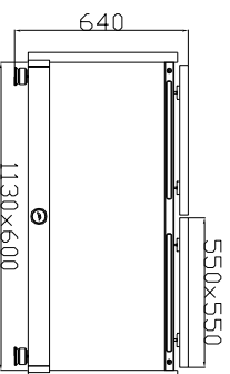
2 LEVELS, 4 COMPONENTS RACK CODE: DS-10THASE-WBR 1+2
