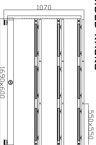
4 LEVELS, 12 COMPONENTS RACK CODE: TS-10THASE-WBR 1+3+3+3
