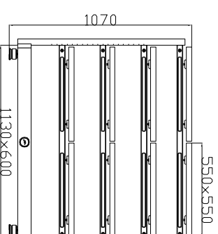
5 LEVELS, 10 COMPONENTS RACK CODE: DS-10THASE-WBR 1+2+2+2+2
