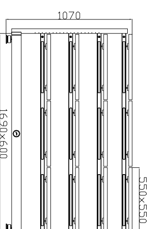
5 LEVELS, 15 COMPONENTS RACK CODE: TS-10THASE-WBR 1+3+3+3+3
