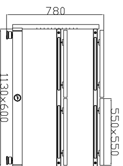
3 LEVELS, 6 COMPONENTS RACK CODE: DS-10THASE-WBR 1+2+2
