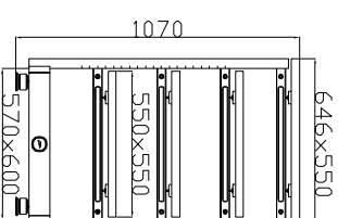
5 LEVELS, 5 COMPONENTS RACK CODE: SS-10THASE-WBR 1+1+1+1+1
