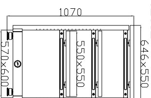
4 LEVELS, 4 COMPONENTS RACK CODE: SS-10THASE-WBR 1+1+1+1
