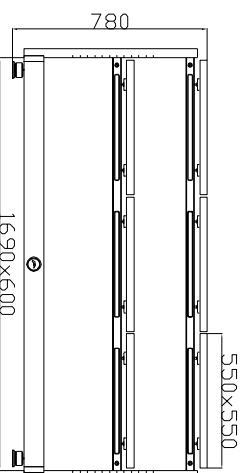
3 LEVELS, 9 COMPONENTS RACK CODE: TS-10THASE-WBR 1+3+3
