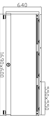
2 LEVELS, 6 COMPONENTS RACK CODE: TS-10THASE-WBR 1+3
