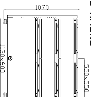
4 LEVELS, 8 COMPONENTS RACK CODE: DS-10THASE-WBR 1+2+2+2
